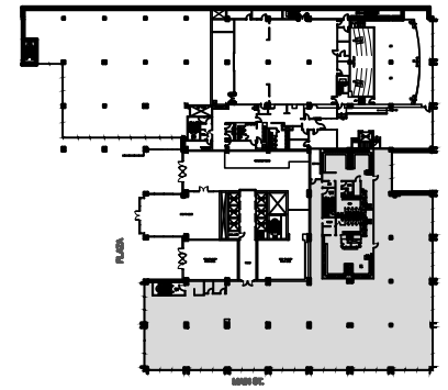
MEZZANINE KEY PLAN
