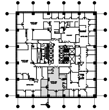
8TH FLOOR KEY PLAN
